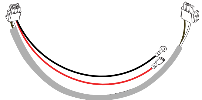
Bluetooth Harness
