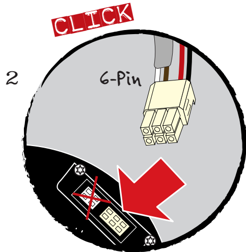
Connect 6 PIN connector blower motor
