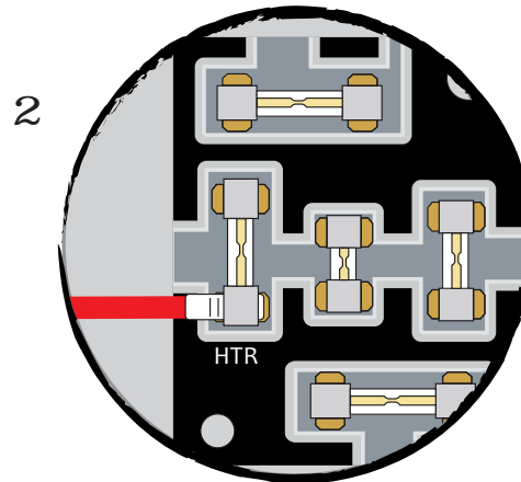
12v Power IGNITION SOURCE (20 amp fuse) (FUSE BLOCK)
