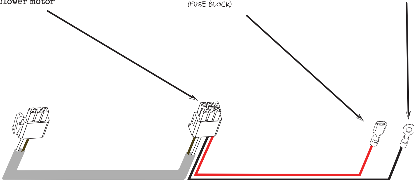
Connect 6 PIN connector blower motor
